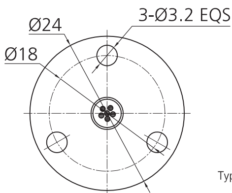
M125C(Type C flange drawing)
