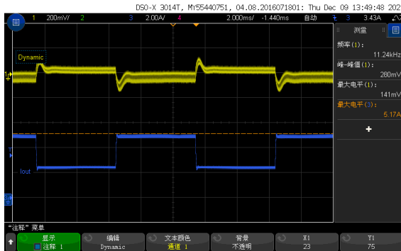
Figure 4, 25% - 50% load dynamic
