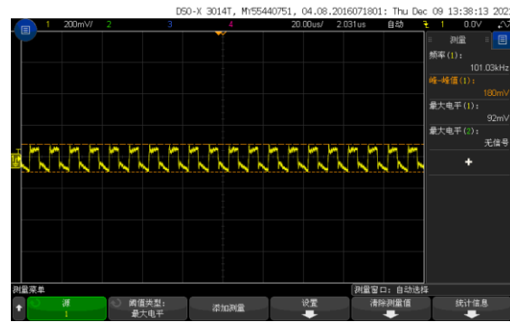
Figure 7, Output ripple & noise (Iout = 10A)
