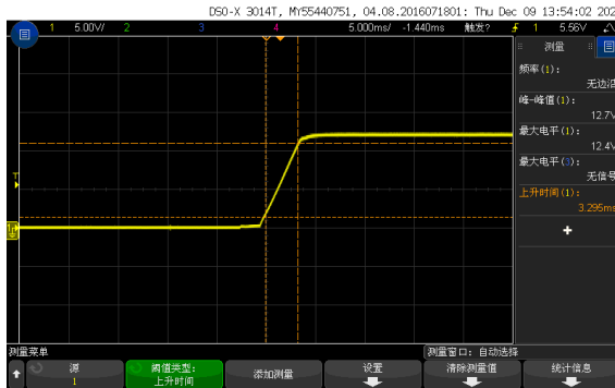
Figure 6, Output voltage established (Iout = 10A)
