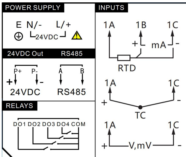
Figure 5 24V Wiring diagram
