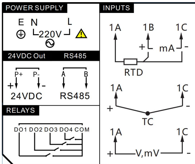
Figure 6 220V Wiring diagram
