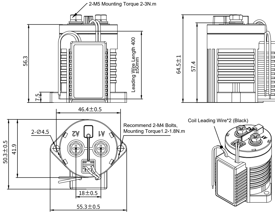
ADH100 With Auxiliary Switch
