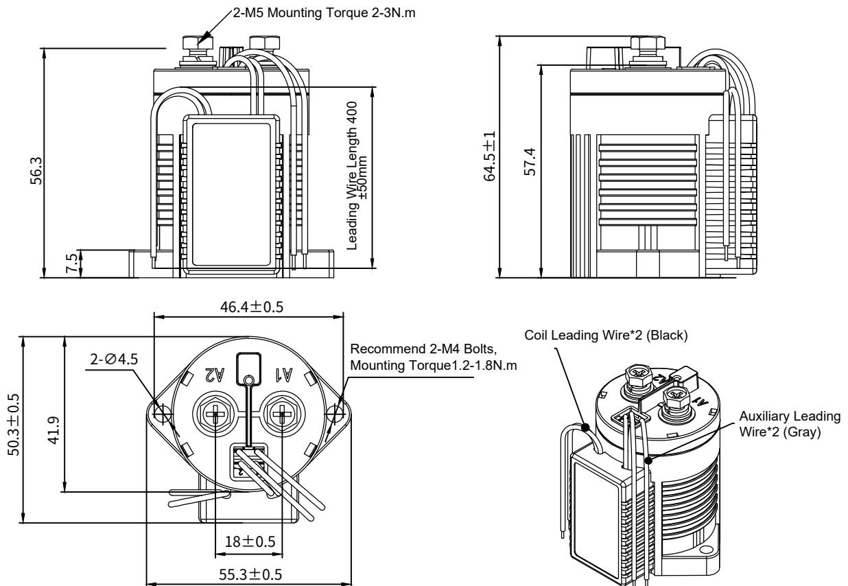
ADH100 With Auxiliary Switch
