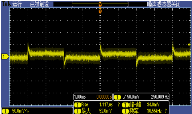
Figure 4, 25% - 50% load dynamic
