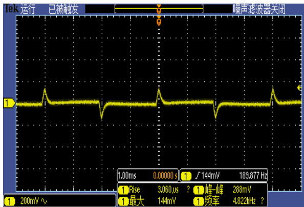
Figure 4, 25% - 50% load dynamic
