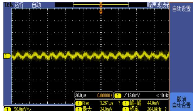
Figure 7, Output ripple & noise (Iout = 40A)
