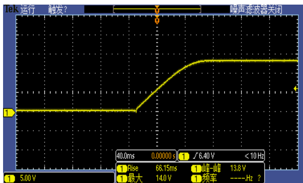
Figure 6, Output voltage established (Iout = 40A)
