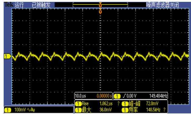
Figure 7, Output ripple & noise (Iout = 5A)
