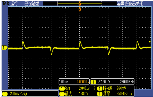
Figure 4, 25% - 50% load dynamic
