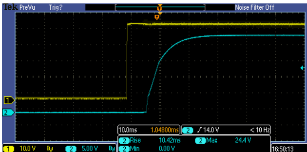
Figure 6, Output voltage established (Iout = 5A)
