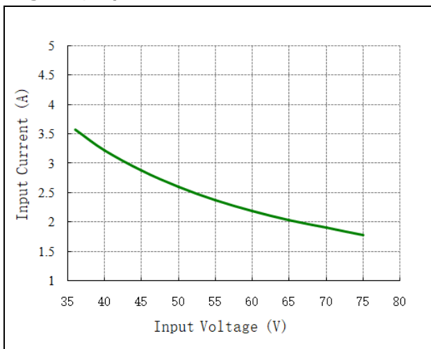
Figure 3, Input V-I
