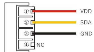
Figure 6. AM2305B Wiring Diagram
